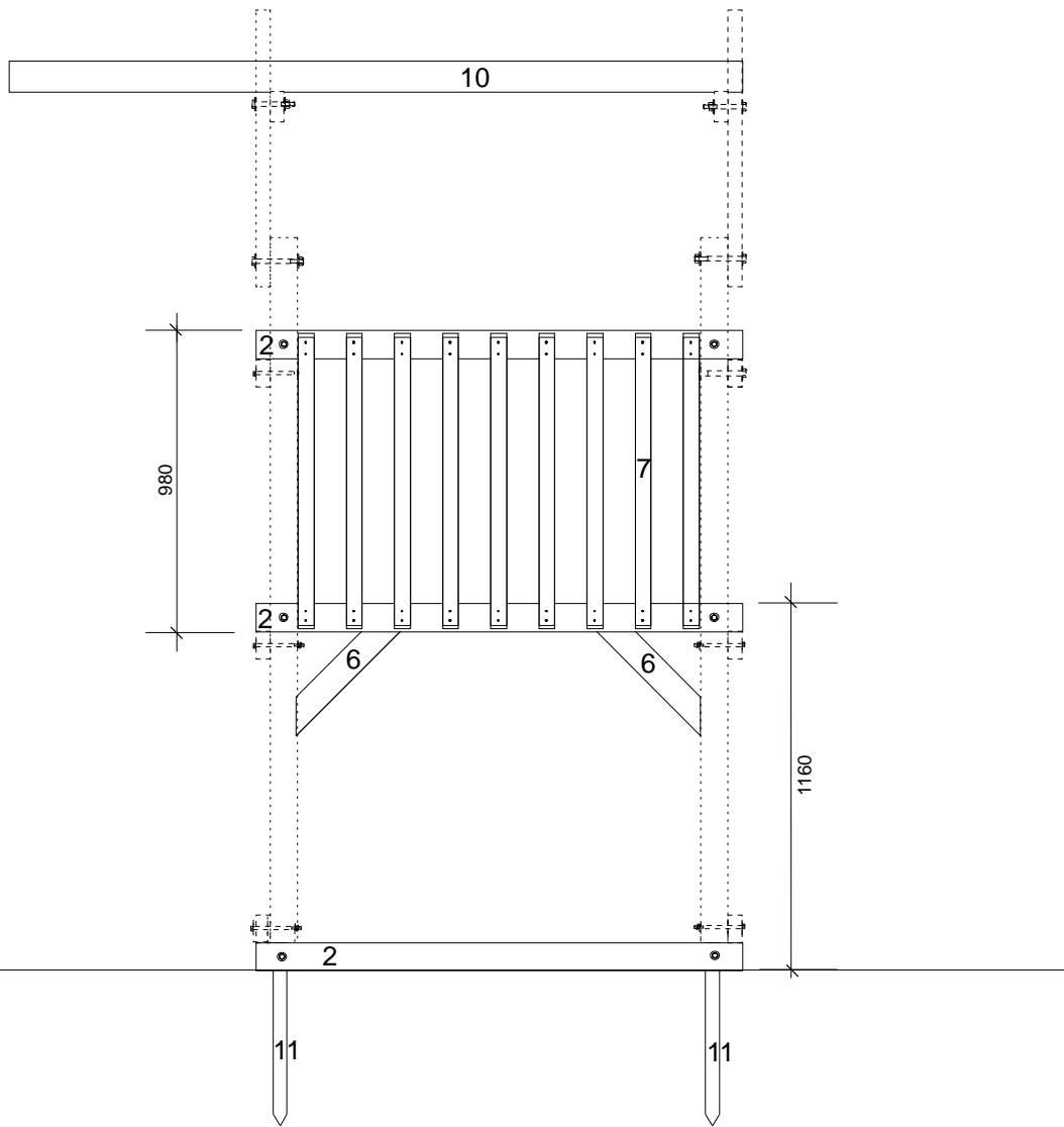
2 90 X 45 FRAMING X 3
